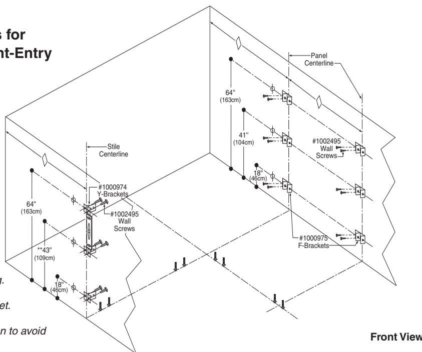
Fig. 4b: Mounting Brackets for Front-Entry Corner Layout.
