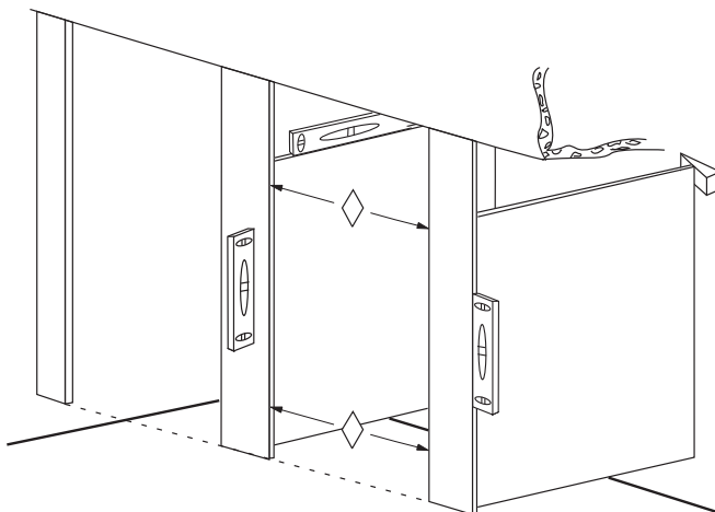
Fig. 9c: Ceiling-Hung Installation.
