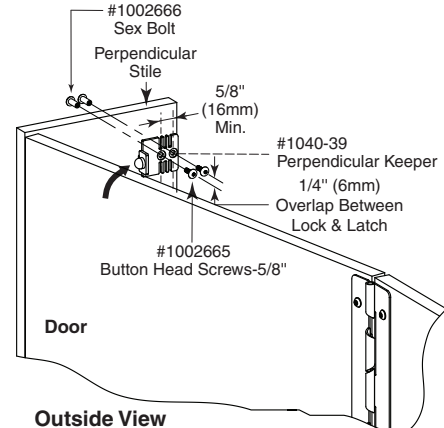
Outside View
