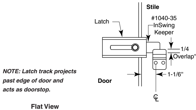
Fig. 10g: INSWING Door Keeper for Perpendicular Stiles.
