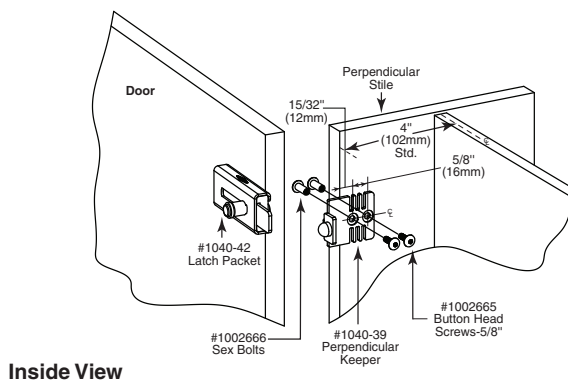
Fig. 10g: INSWING Door Keeper for Perpendicular Stiles.
