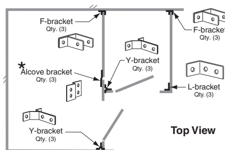
Fig. 4c: Mounting Brackets for Closed Alcove with Adjoining Front-Entry Stall.
