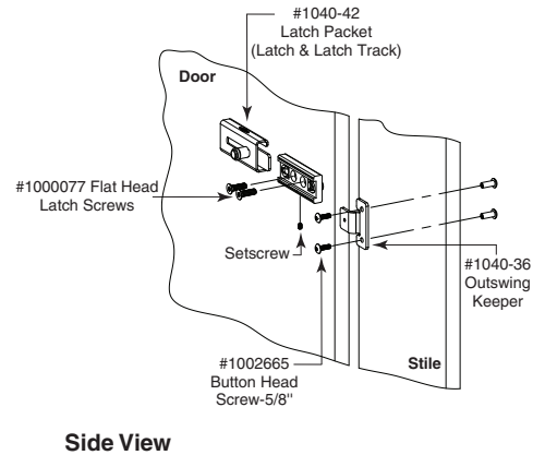
Fig. 10f: OUTSWING Door Keeper for Inline Stiles.
