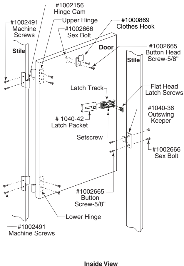
Fig. 10b: OUTSWING Door Hardware. (example)
