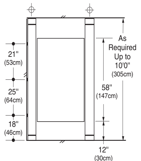
Fig. 6c: Floor-to-Ceiling Anchored.
