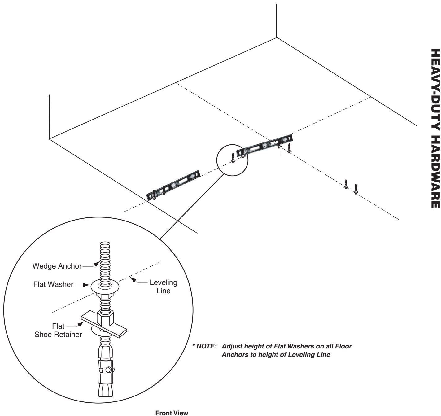
Fig. 3: Rough Leveling Floor Anchors.
