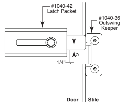
Fig. 10h: OUTSWING Door Keeper for Perpendicular Stiles.
