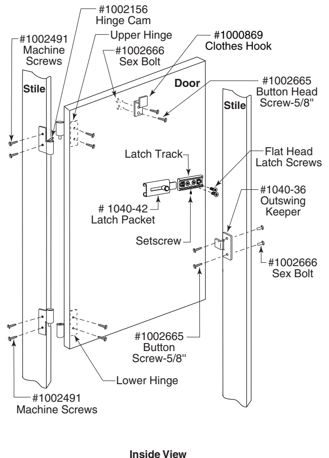
Fig. 10b: OUTSWING Door Hardware. (example)
